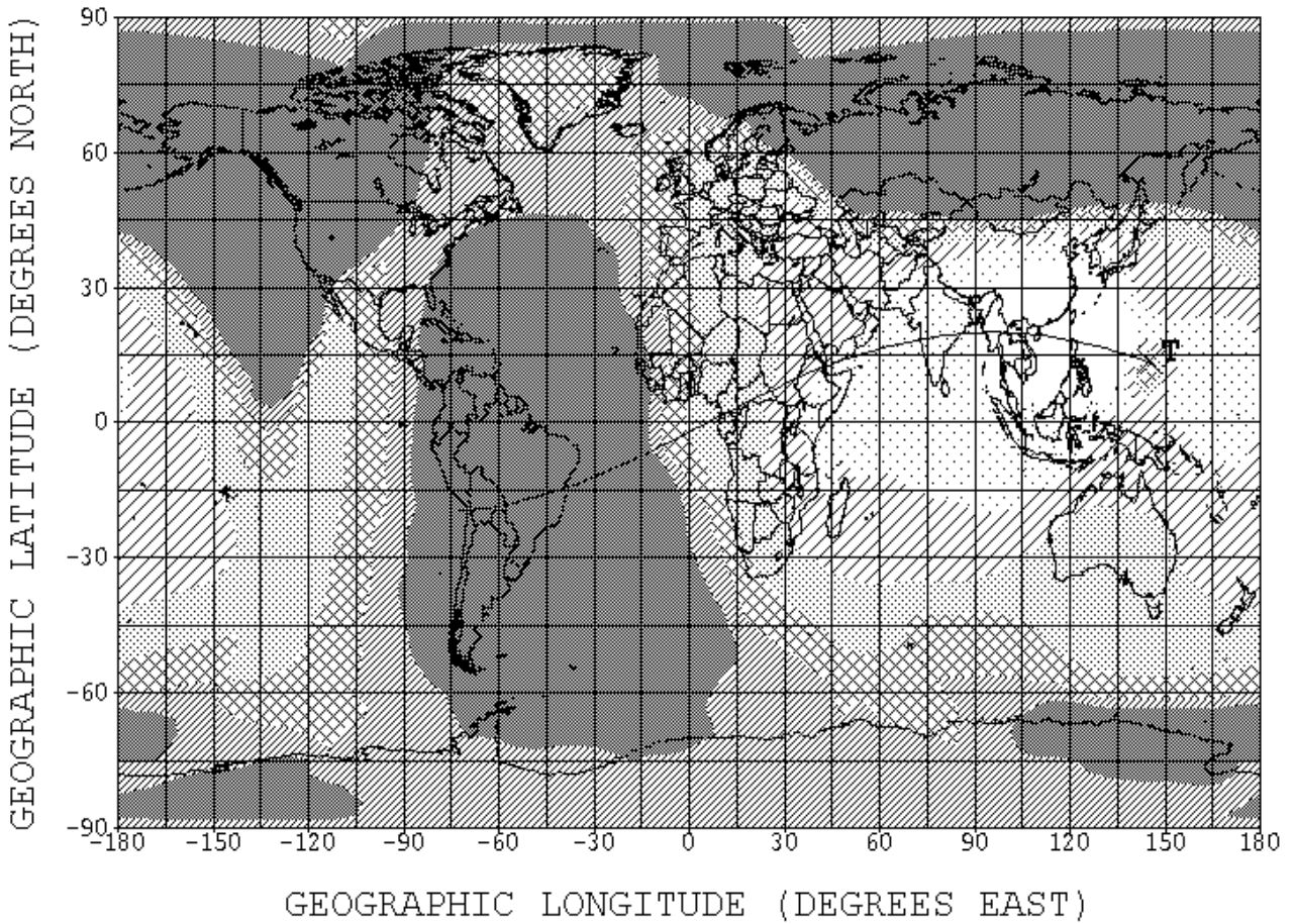
Pic.3: KTWR - Guam at 1500 UTC on 15330 kHz, beam 285 degrees.
